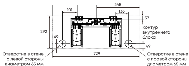
MDSAL-12HRFN8
