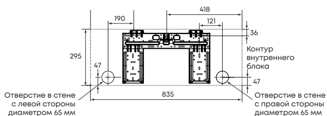
MDSAL-18HRFN8
