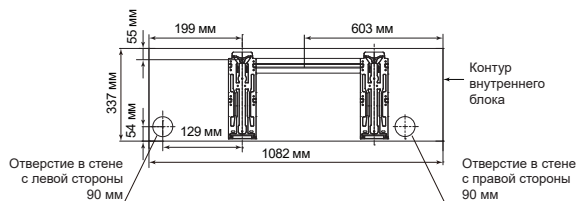
MDSAL-24HRFN8
