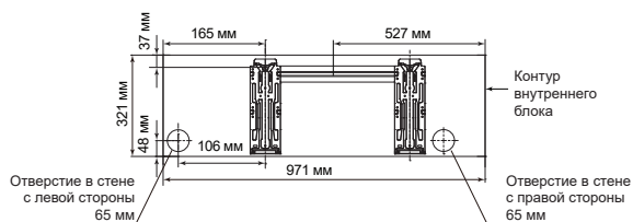
MDSAL-24HRFN8
